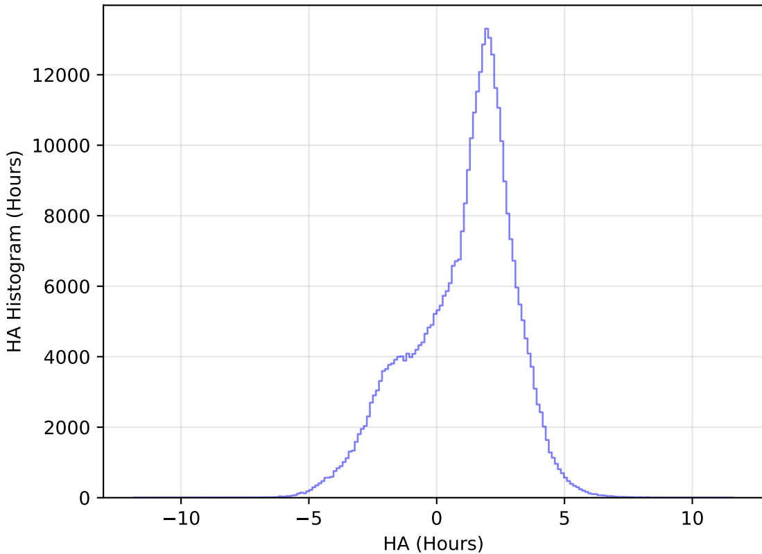
too_elab_r8_d2_griz_v3.4_10yrs WFD y band: HA Histogram
