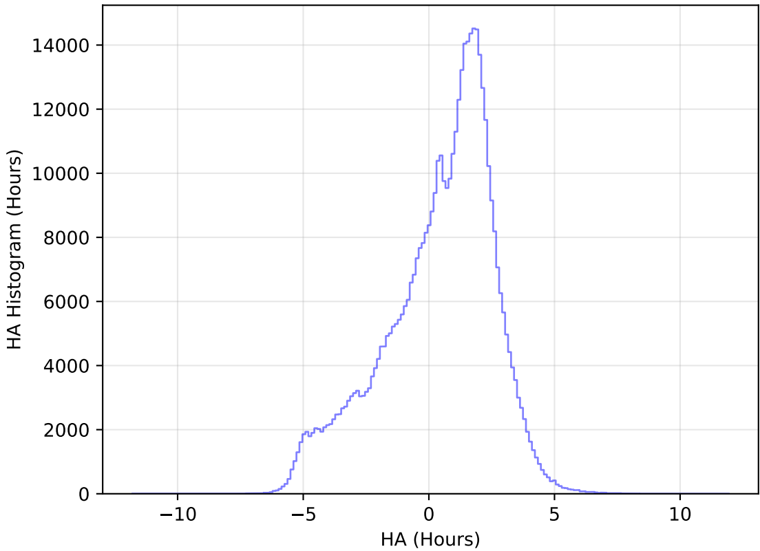
too_elab_r8_d2_griz_v3.4_10yrs WFD r band: HA Histogram
