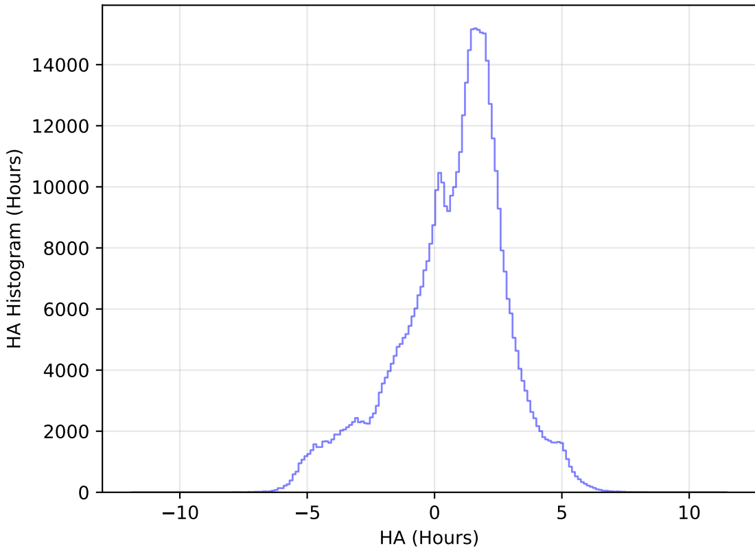
too_elab_r8_d2_griz_v3.4_10yrs WFD i band: HA Histogram
