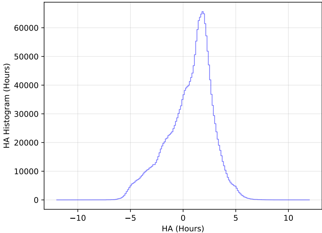
too_elab_r8_d2_griz_v3.4_10yrs WFD all bands: HA Histogram
