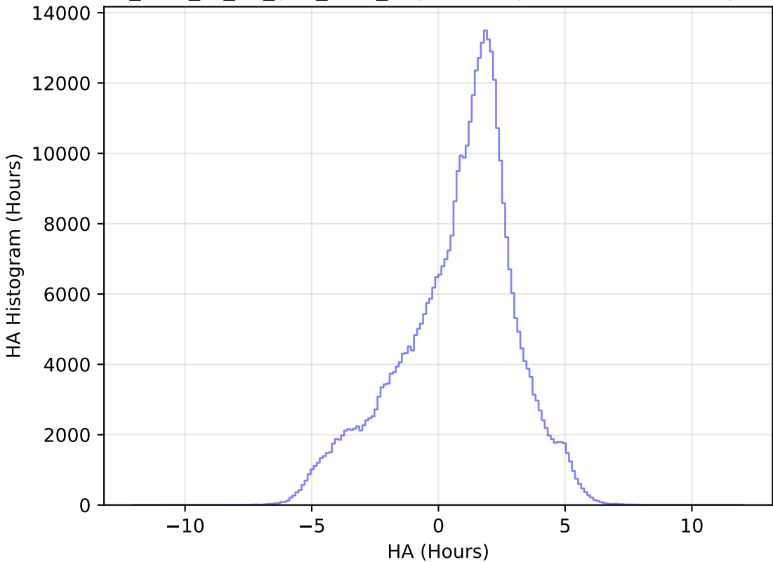
too_elab_r8_d2_griz_v3.4_10yrs All sky z band: HA Histogram
