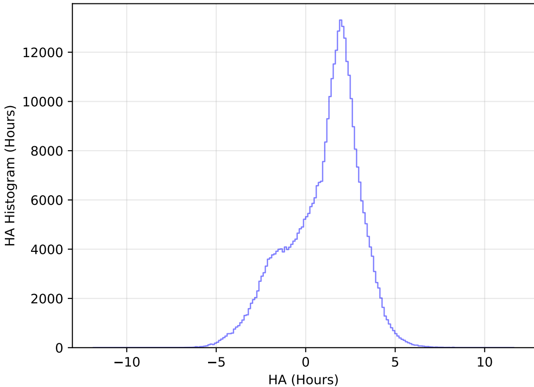
too_elab_r8_d2_griz_v3.4_10yrs All sky y band: HA Histogram
