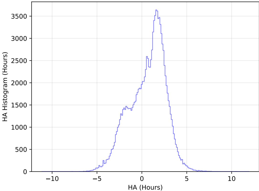
too_elab_r8_d2_griz_v3.4_10yrs All sky u band: HA Histogram
