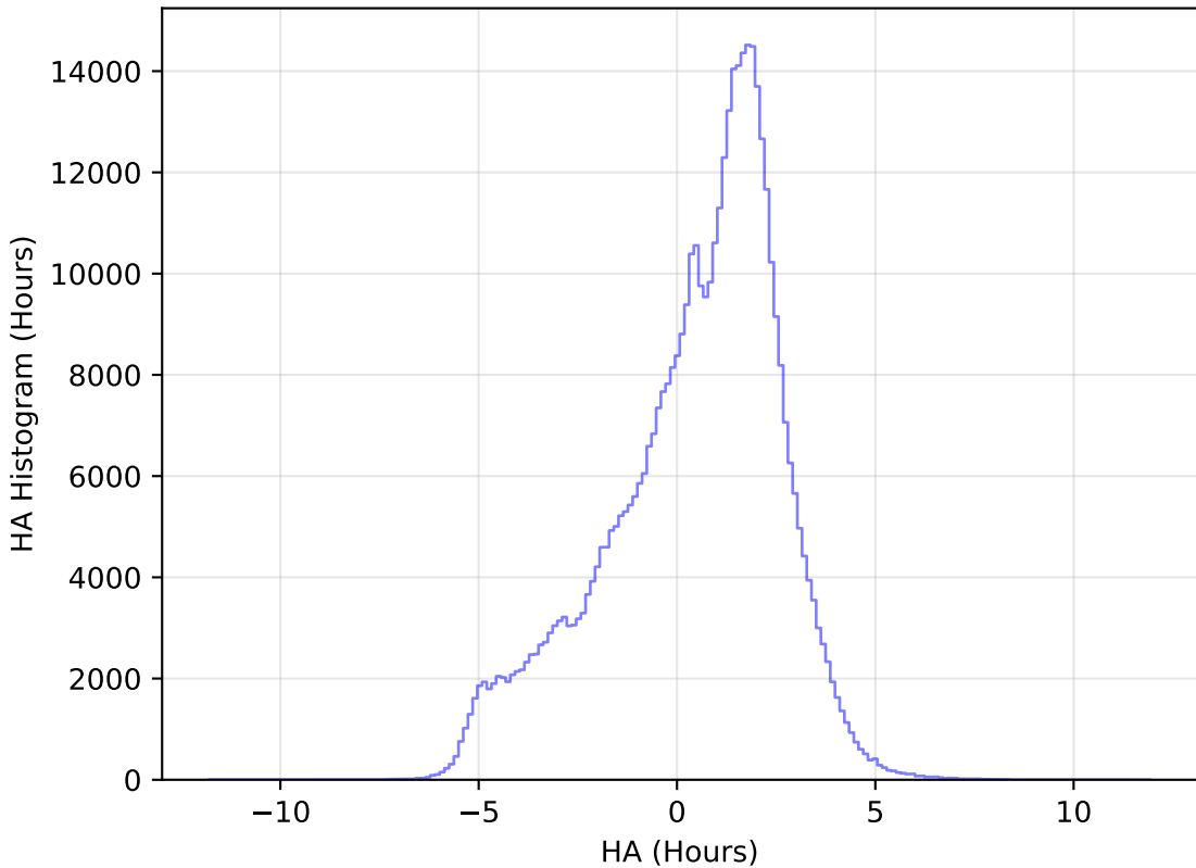
too_elab_r8_d2_griz_v3.4_10yrs All sky r band: HA Histogram
