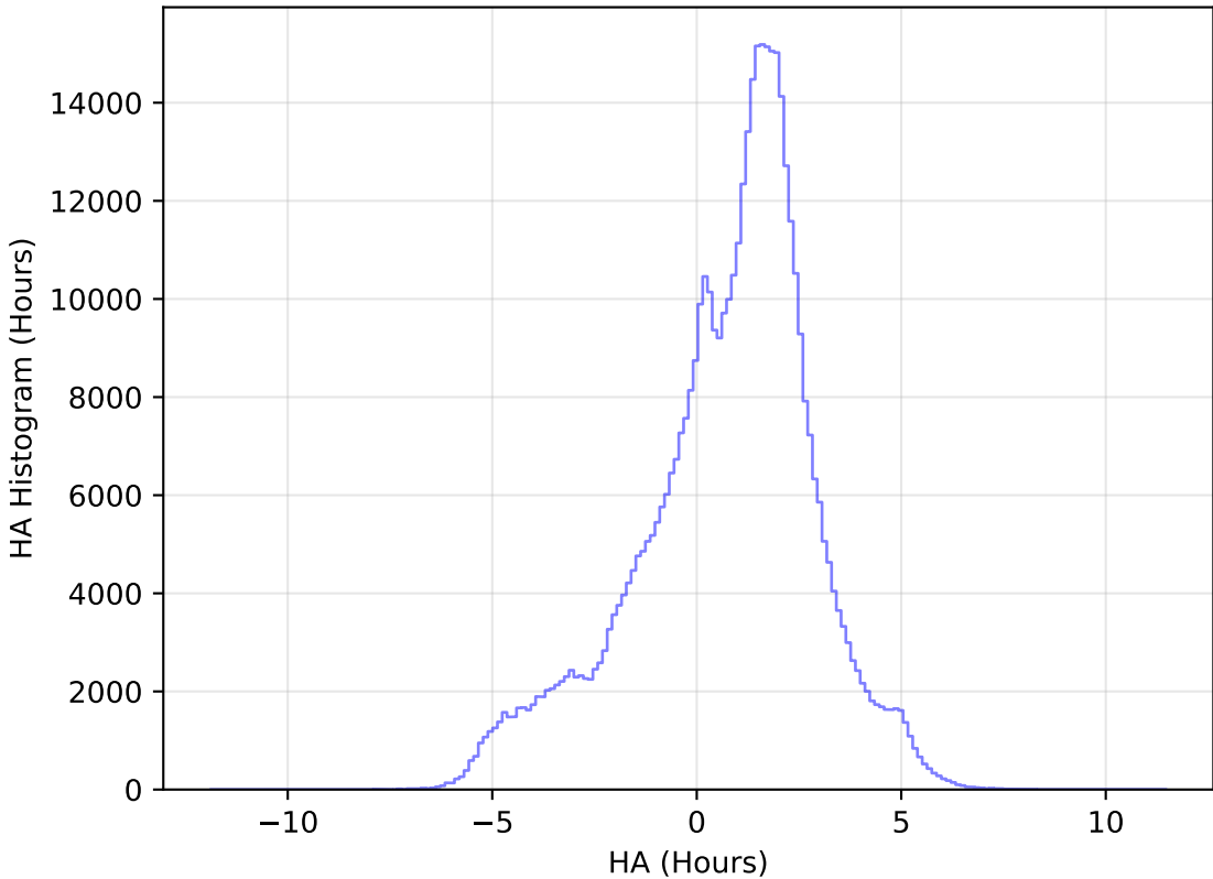
too_elab_r8_d2_griz_v3.4_10yrs All sky i band: HA Histogram
