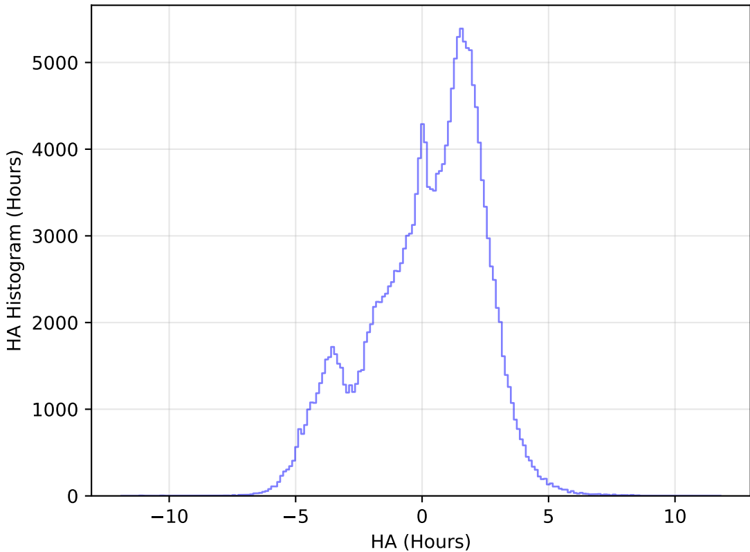
too_elab_r8_d2_griz_v3.4_10yrs All sky g band: HA Histogram
