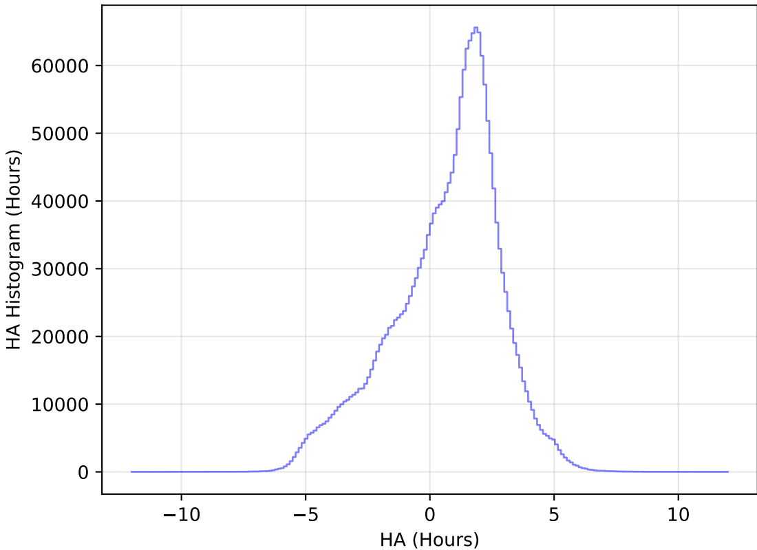
too_elab_r8_d2_griz_v3.4_10yrs All sky all bands: HA Histogram
