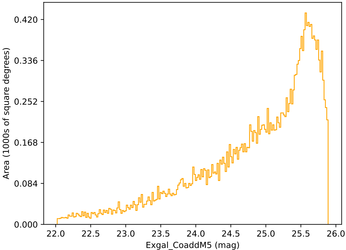
too_elab_r8_d2_griz_v3.4_10yrs Yr 3-4 r band: Exgal_CoaddM5
