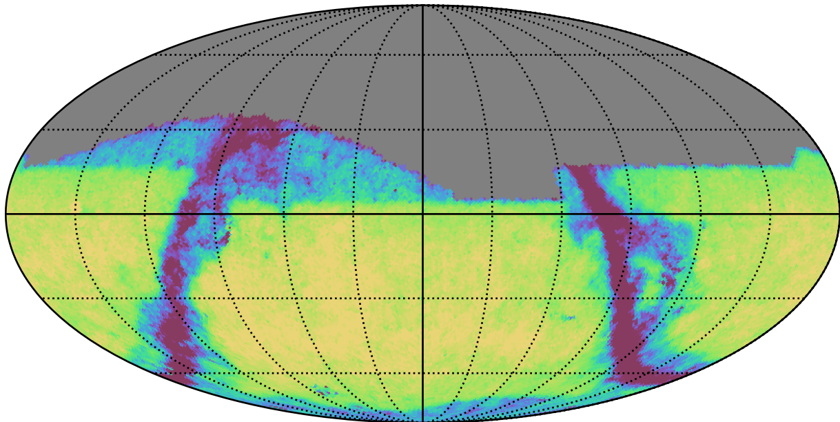
too_elab_r8_d2_griz_v3.4_10yrs Yr 1 i band: Exgal_CoaddM5
