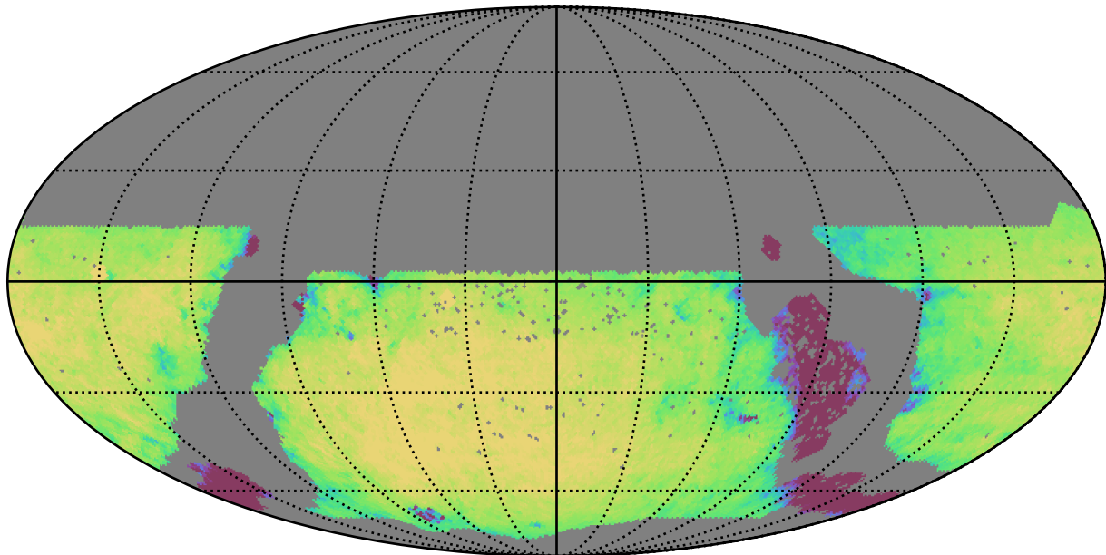
too_elab_r8_d2_griz_v3.4_10yrs WFD u band: Exgal_CoaddM5
