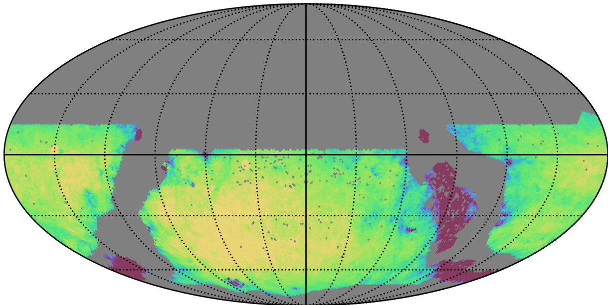
too_elab_r8_d2_griz_v3.4_10yrs WFD g band: Exgal_CoaddM5
