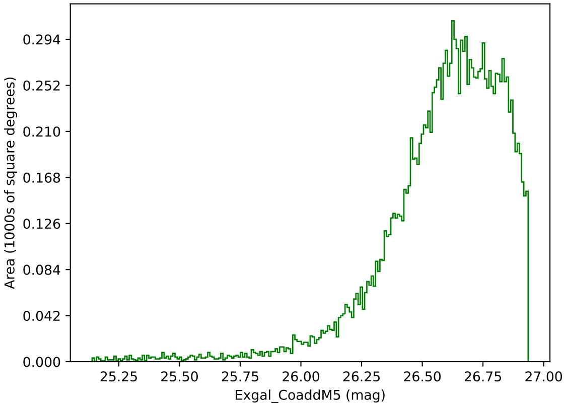
too_elab_r8_d2_griz_v3.4_10yrs WFD g band: Exgal_CoaddM5
