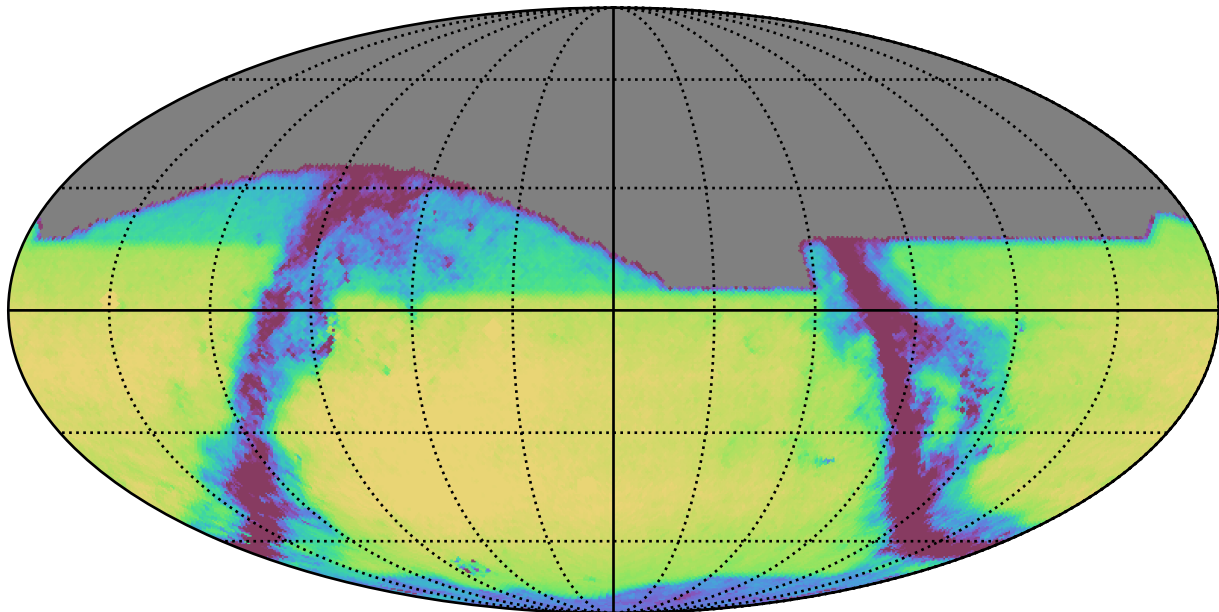
too_elab_r8_d2_griz_v3.4_10yrs All sky i band: Exgal_CoaddM5
