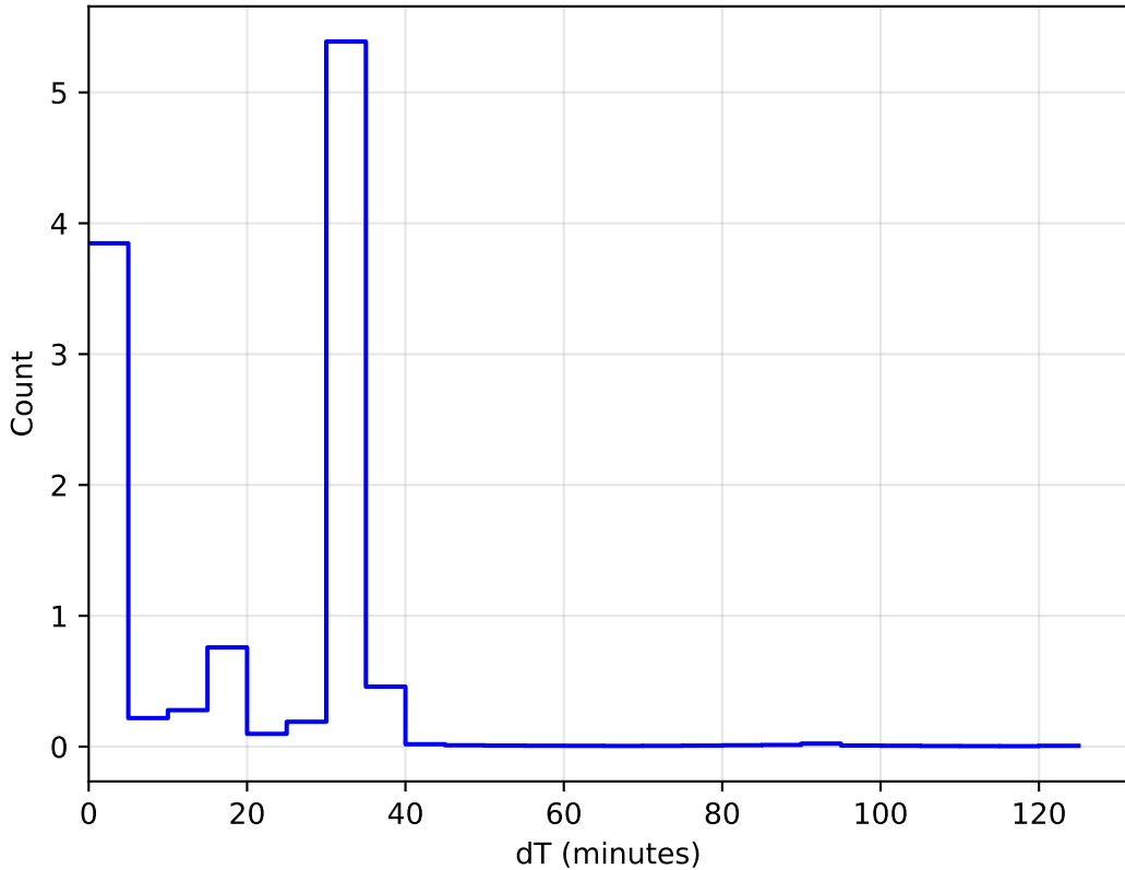
too_elab_r8_d2_griz_v3.4_10yrs WFD: DeltaT Histogram
