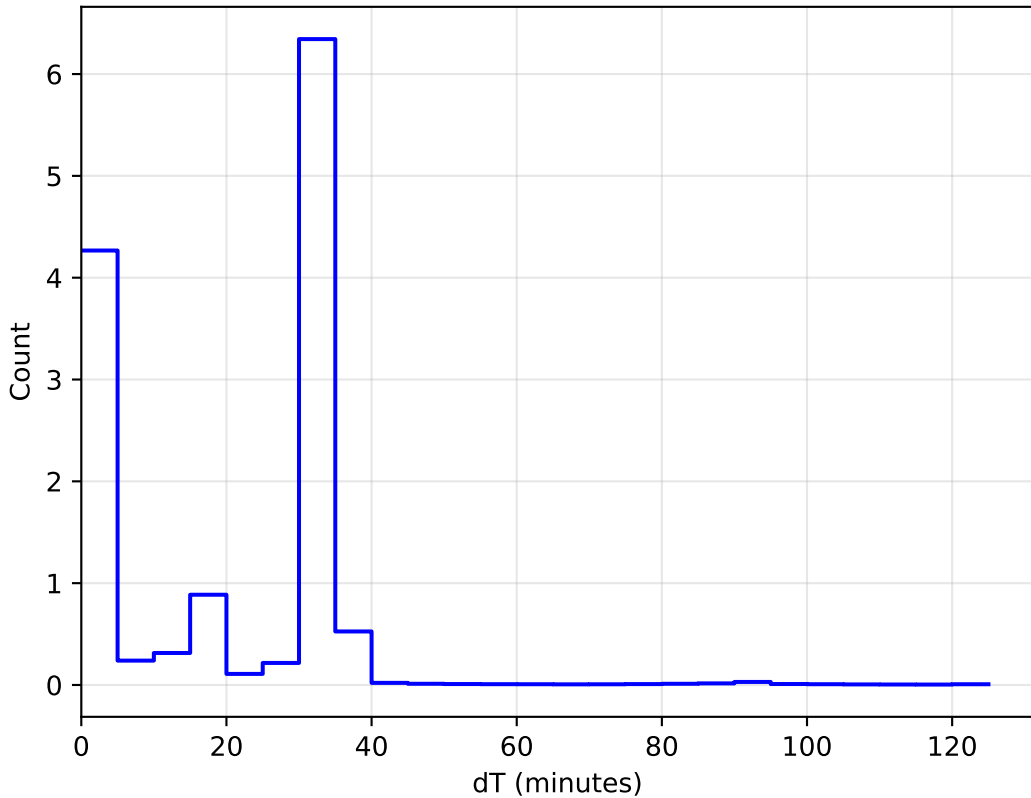
too_elab_r8_d2_griz_v3.4_10yrs All sky: DeltaT Histogram 1e6
