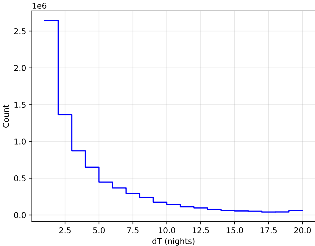
too_elab_r8_d2_griz_v3.4_10yrs WFD all bands: DeltaNight Histogram
