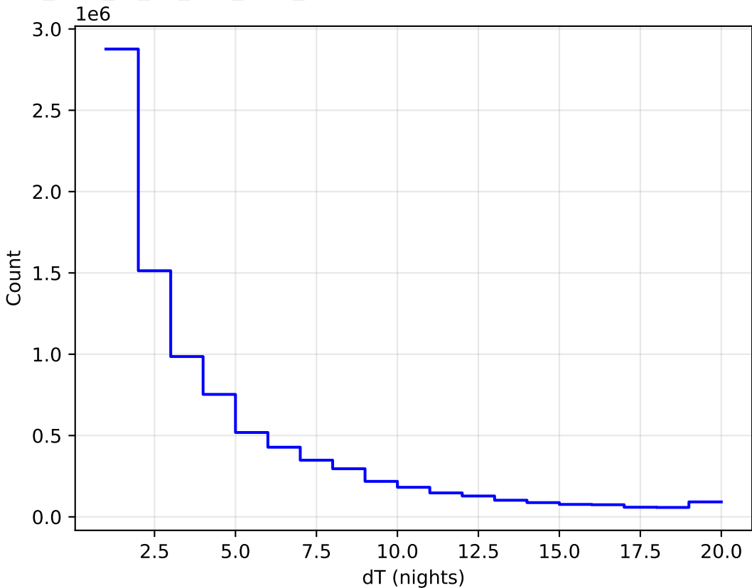
too_elab_r8_d2_griz_v3.4_10yrs All sky all bands: DeltaNight Histogram
