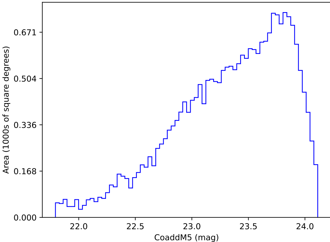
too_elab_r8_d2_griz_v3.4_10yrs Yr 3-4 y band: CoaddM5
