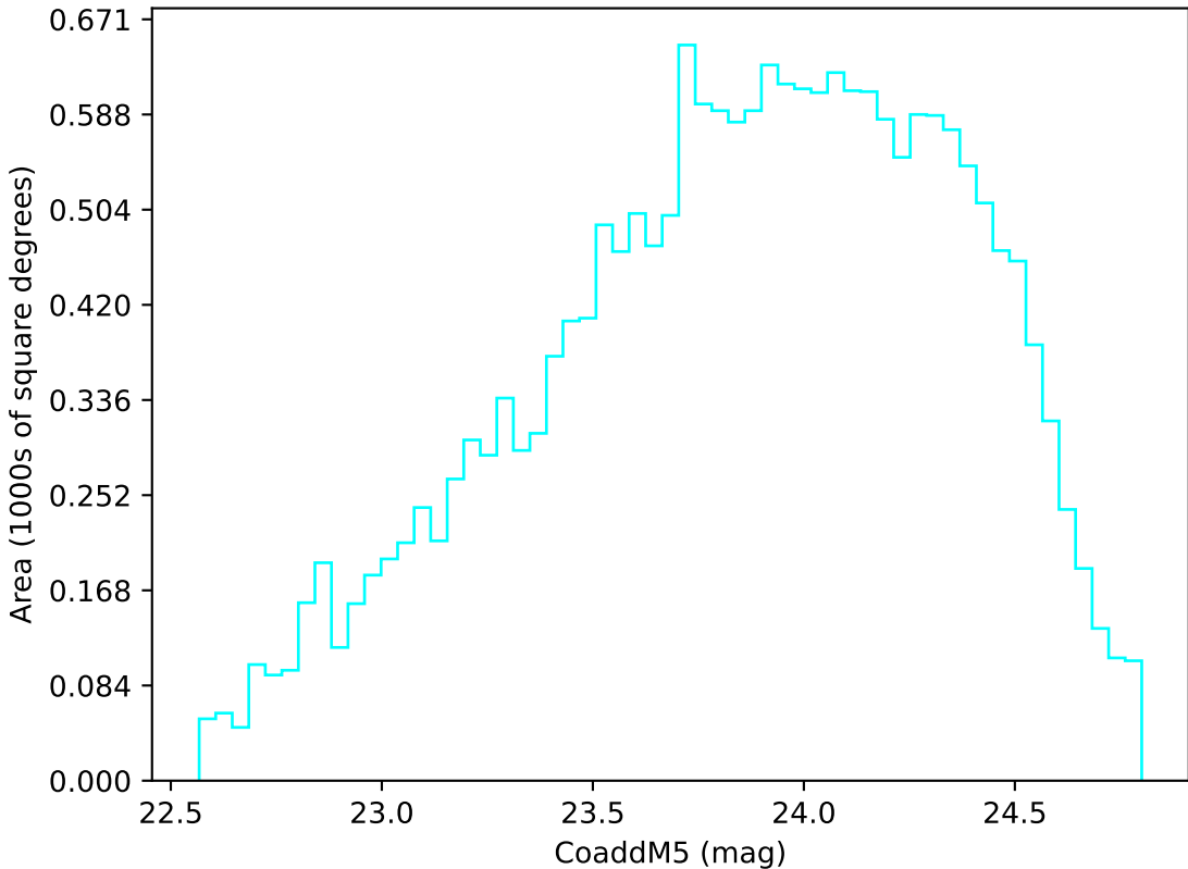
too_elab_r8_d2_griz_v3.4_10yrs Yr 3-4 u band: CoaddM5
