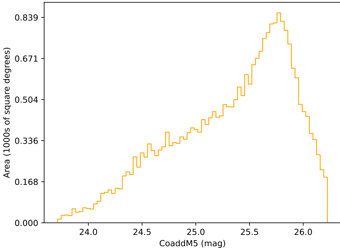
too_elab_r8_d2_griz_v3.4_10yrs Yr 3-4 r band: CoaddM5
