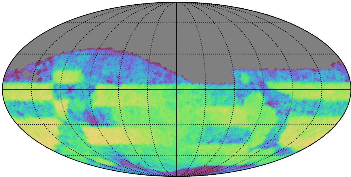
too_elab_r8_d2_griz_v3.4_10yrs Yr 3-4 i band: CoaddM5
