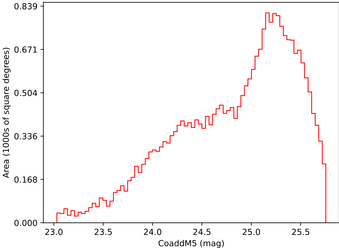
too_elab_r8_d2_griz_v3.4_10yrs Yr 3-4 i band: CoaddM5
