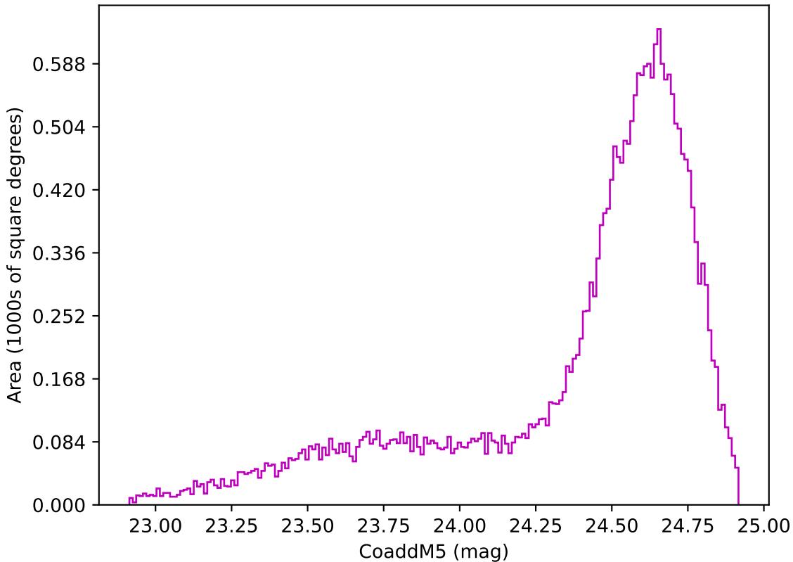
too_elab_r8_d2_griz_v3.4_10yrs Yr 1 z band: CoaddM5
