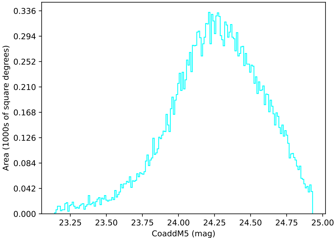
too_elab_r8_d2_griz_v3.4_10yrs Yr 1 u band: CoaddM5
