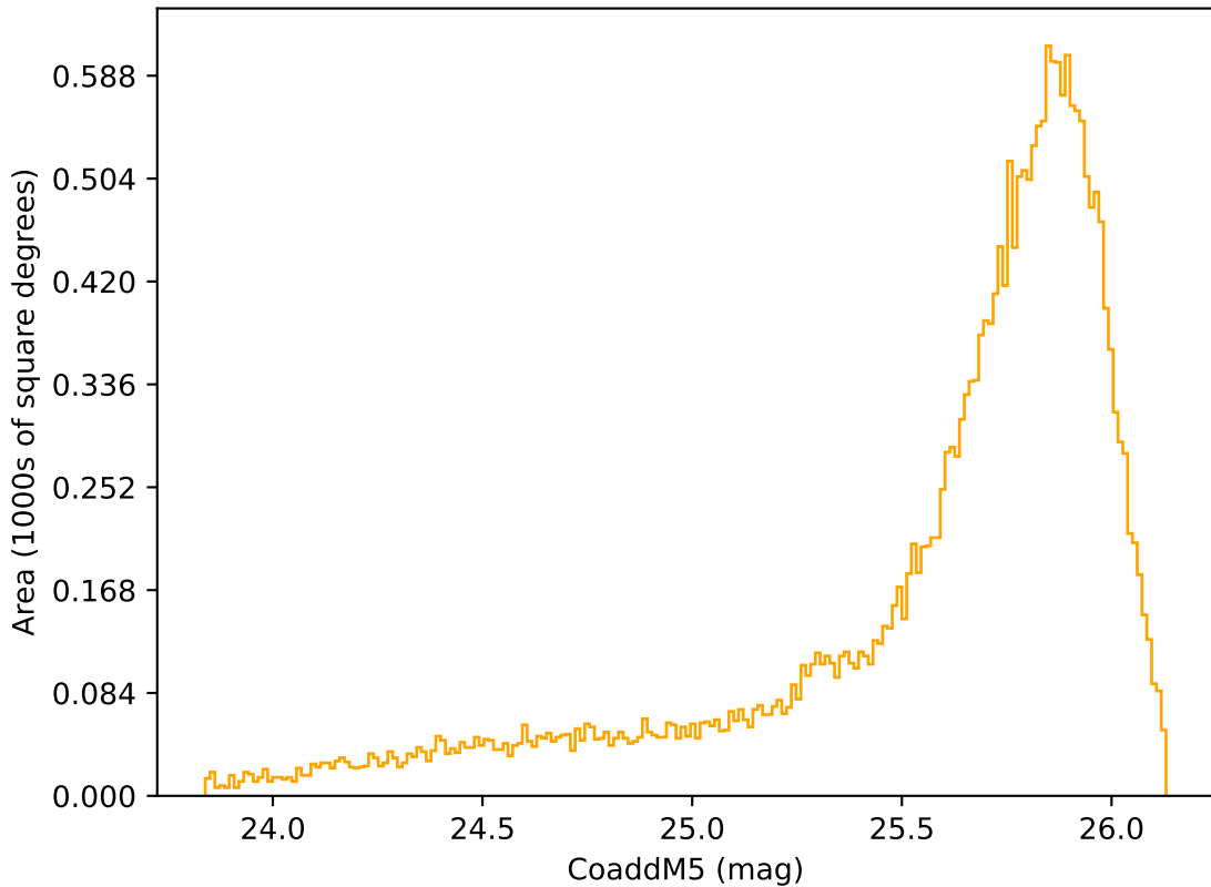
too_elab_r8_d2_griz_v3.4_10yrs Yr 1 r band: CoaddM5
