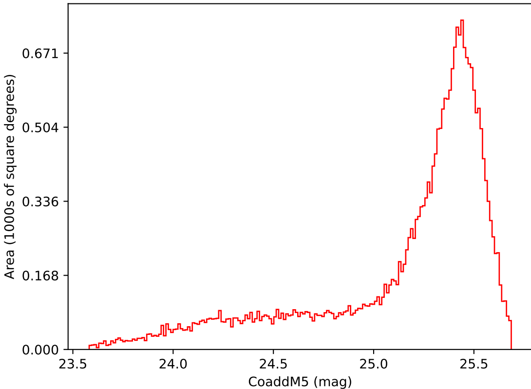
too_elab_r8_d2_griz_v3.4_10yrs Yr 1 i band: CoaddM5
