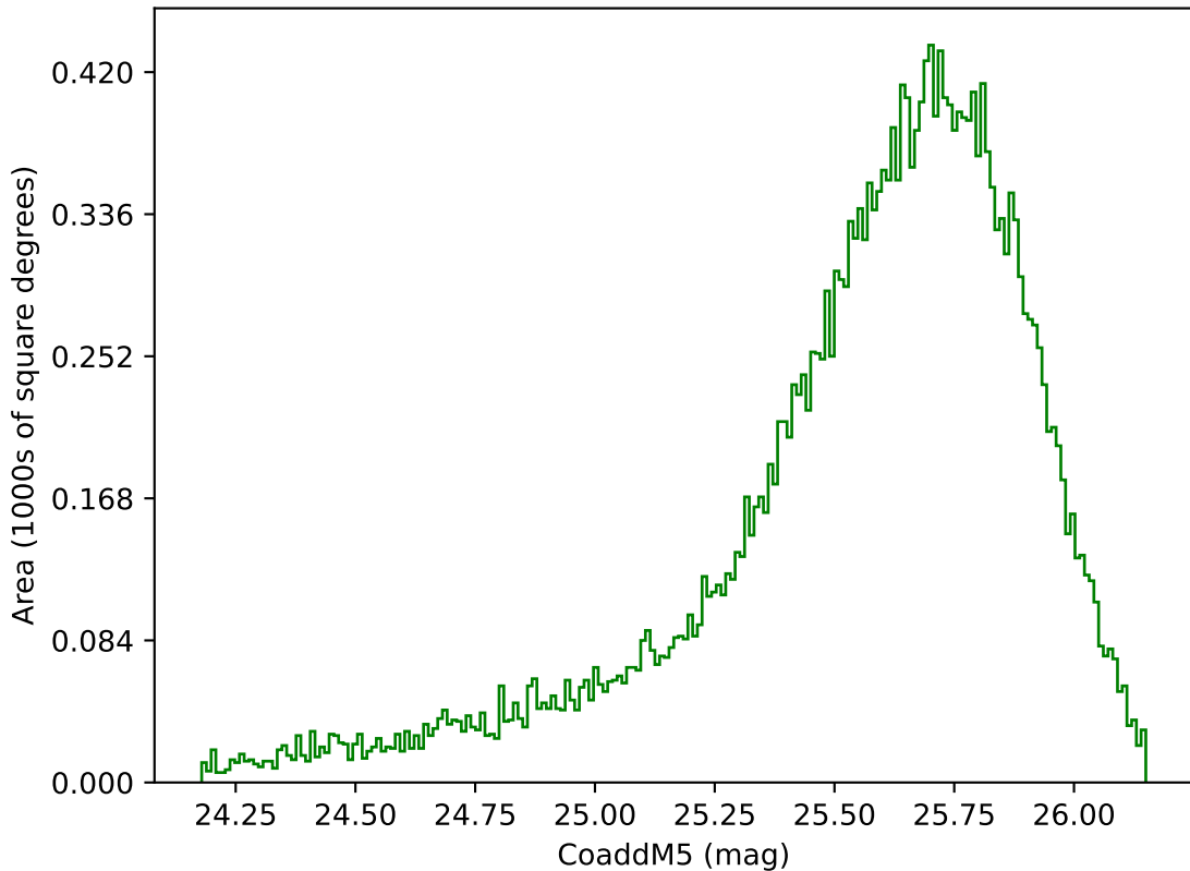
too_elab_r8_d2_griz_v3.4_10yrs Yr 1 g band: CoaddM5
