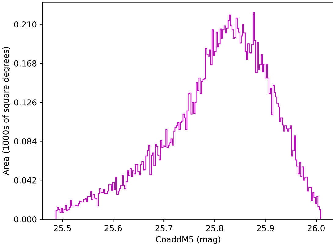
too_elab_r8_d2_griz_v3.4_10yrs WFD z band: CoaddM5
