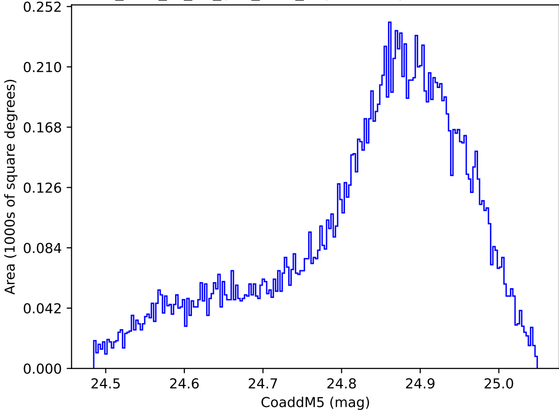
too_elab_r8_d2_griz_v3.4_10yrs WFD y band: CoaddM5
