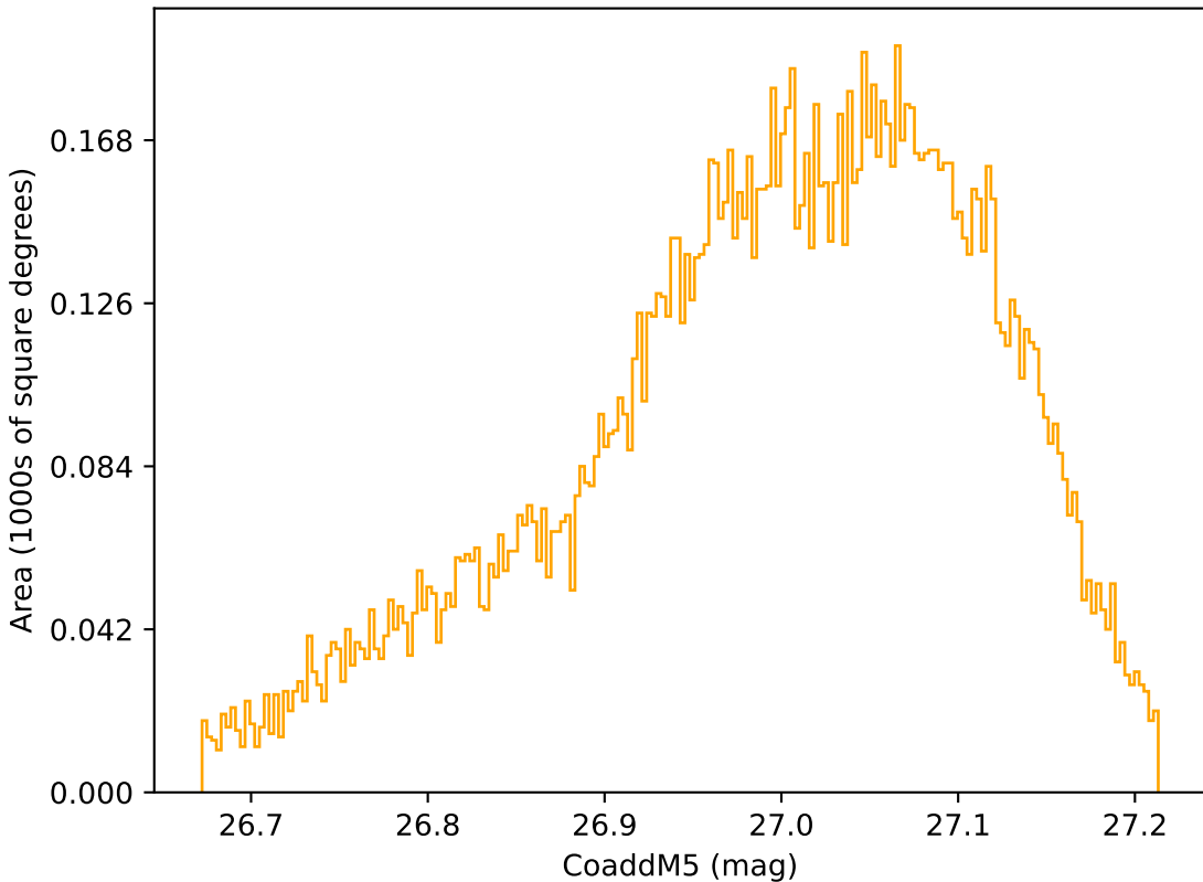
too_elab_r8_d2_griz_v3.4_10yrs WFD r band: CoaddM5
