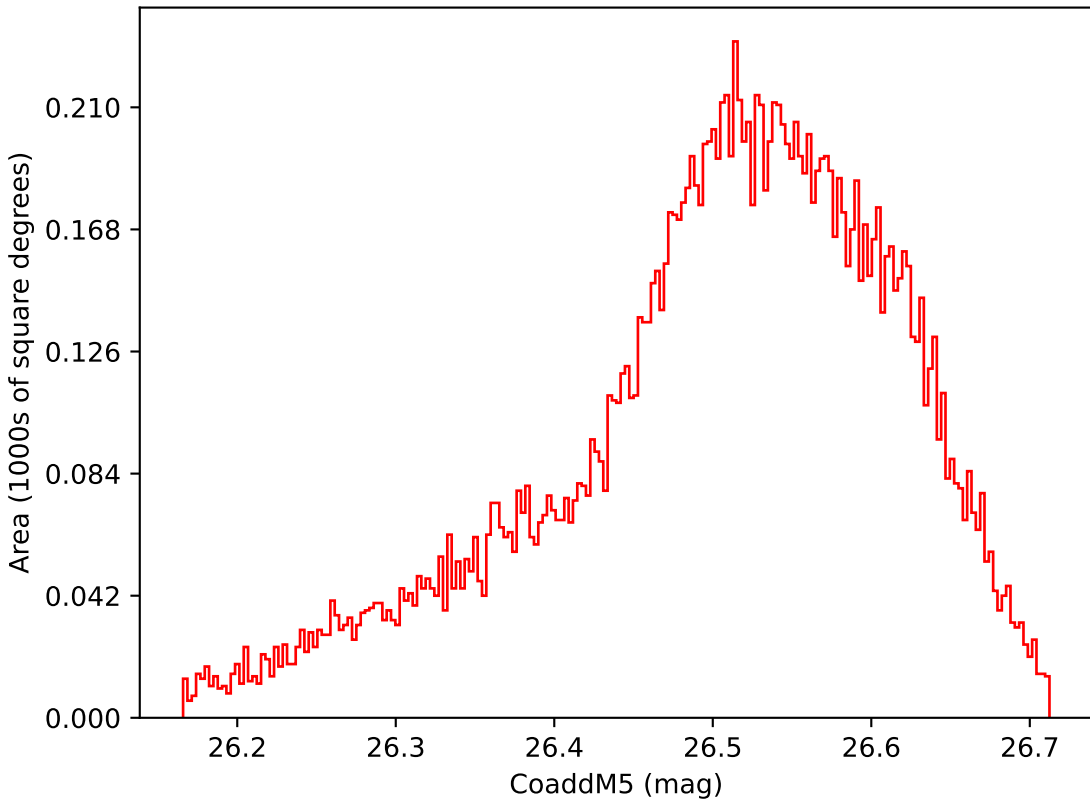
too_elab_r8_d2_griz_v3.4_10yrs WFD i band: CoaddM5
