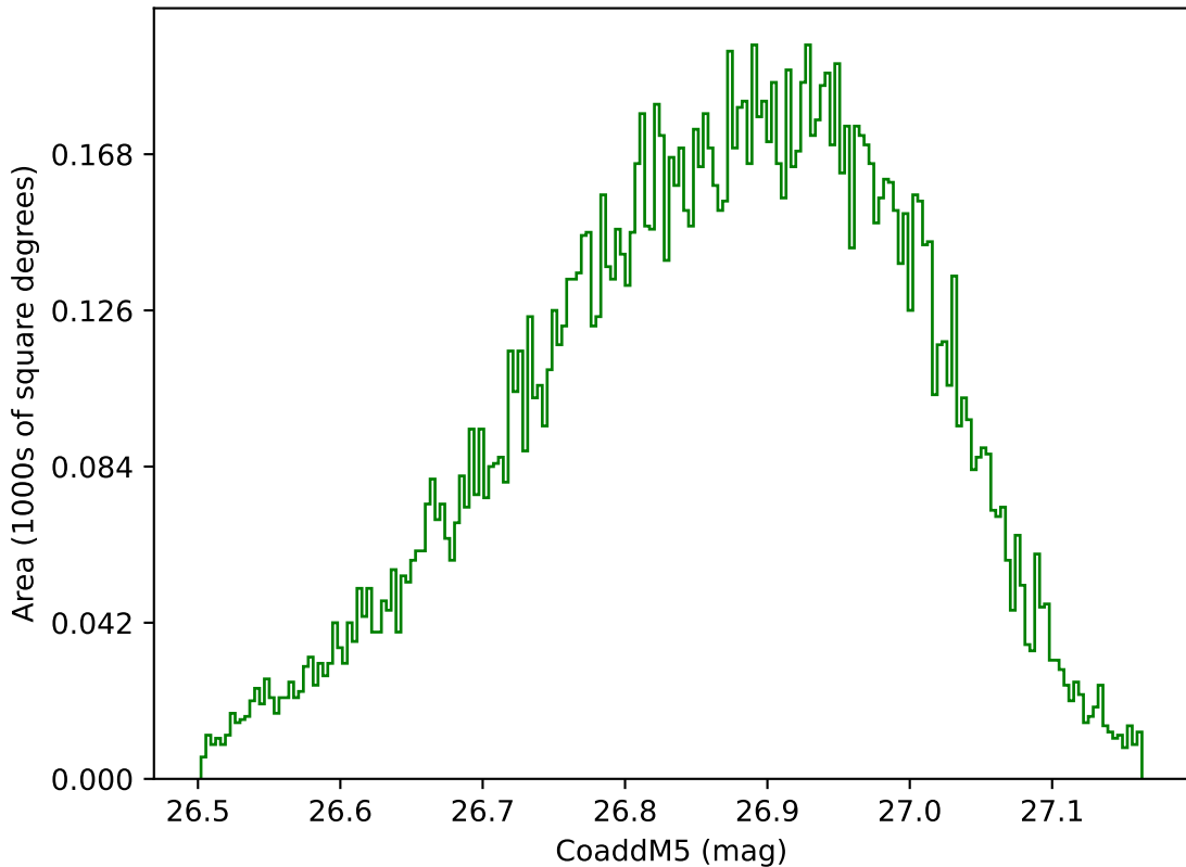
too_elab_r8_d2_griz_v3.4_10yrs WFD g band: CoaddM5
