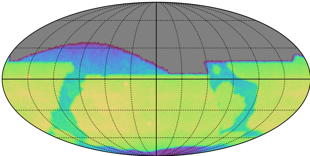
too_elab_r8_d2_griz_v3.4_10yrs All sky z band: CoaddM5
