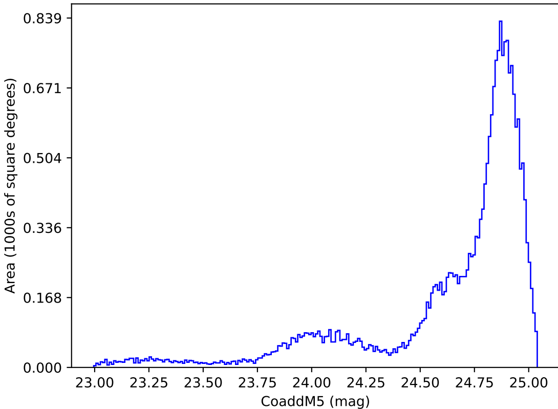
too_elab_r8_d2_griz_v3.4_10yrs All sky y band: CoaddM5
