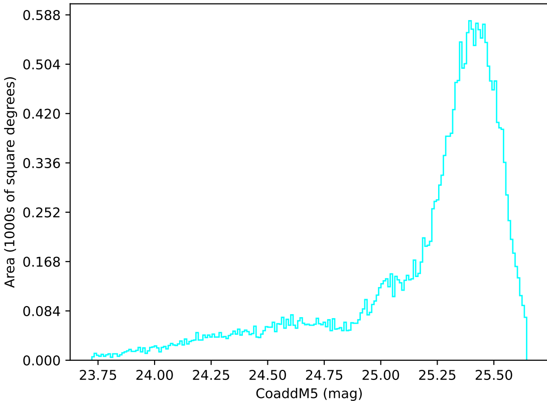
too_elab_r8_d2_griz_v3.4_10yrs All sky u band: CoaddM5
