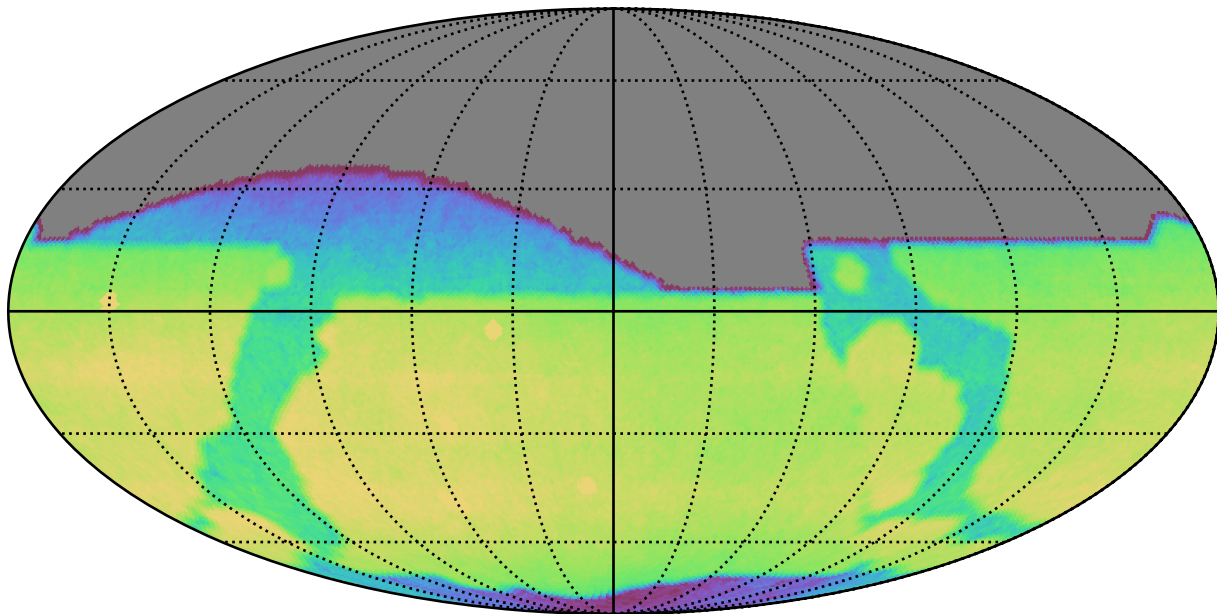
too_elab_r8_d2_griz_v3.4_10yrs All sky r band: CoaddM5
