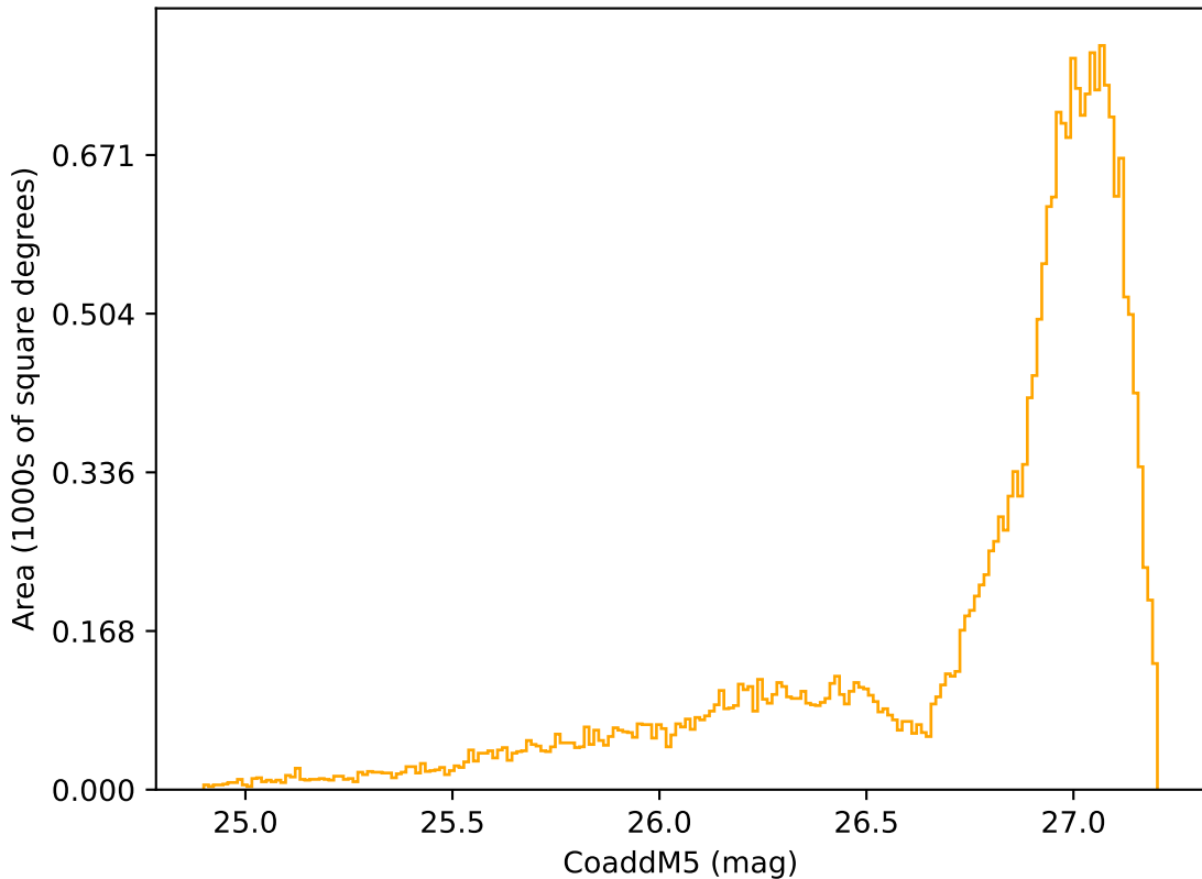
too_elab_r8_d2_griz_v3.4_10yrs All sky r band: CoaddM5
