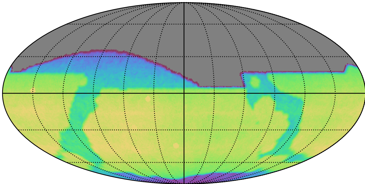
too_elab_r8_d2_griz_v3.4_10yrs All sky i band: CoaddM5
