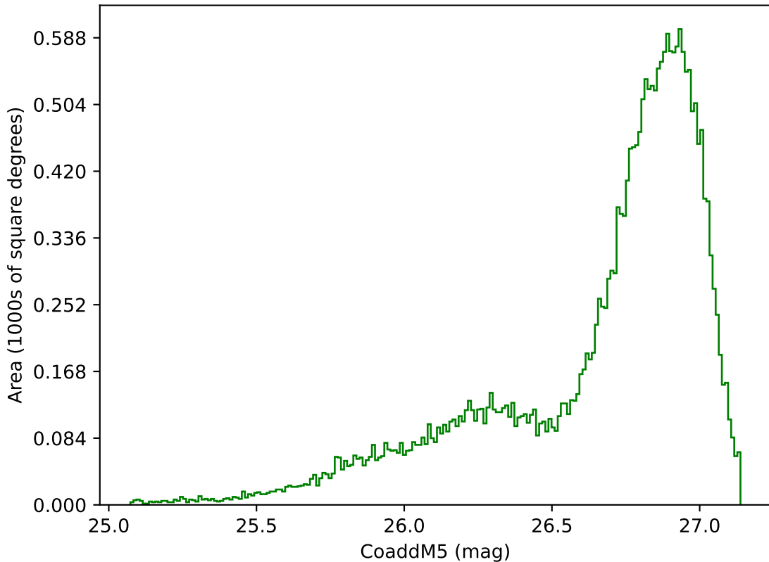
too_elab_r8_d2_griz_v3.4_10yrs All sky g band: CoaddM5
