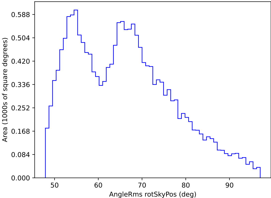
too_elab_r8_d2_griz_v3.4_10yrs WFD r band: AngleRms rotSkyPos
