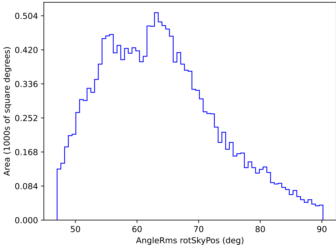
too_elab_r8_d2_griz_v3.4_10yrs WFD i band: AngleRms rotSkyPos
