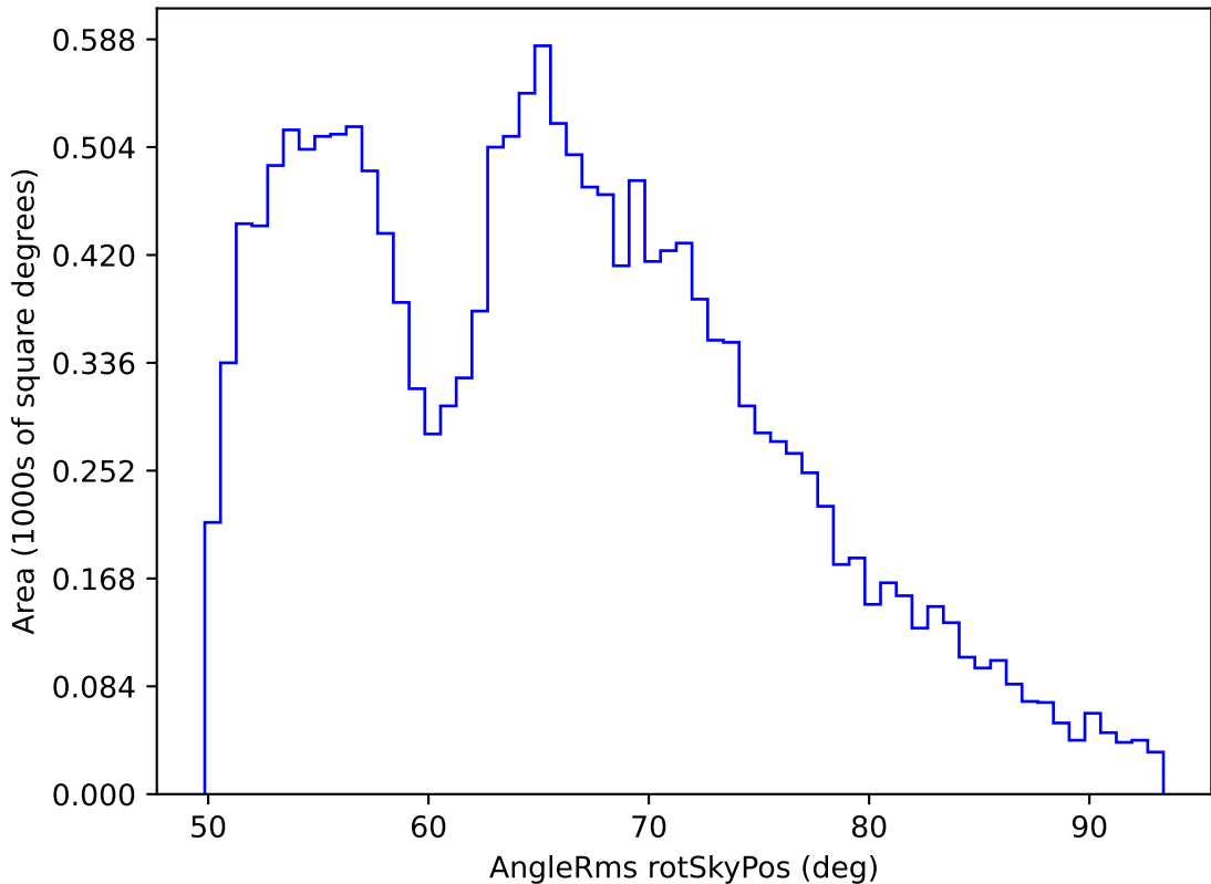
too_elab_r8_d2_griz_v3.4_10yrs WFD all bands: AngleRms rotSkyPos
