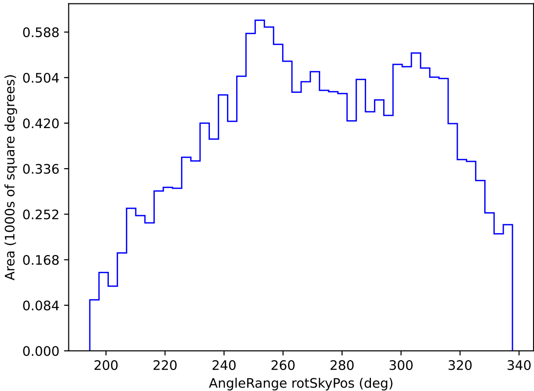
too_elab_r8_d2_griz_v3.4_10yrs WFD y band: AngleRange rotSkyPos
