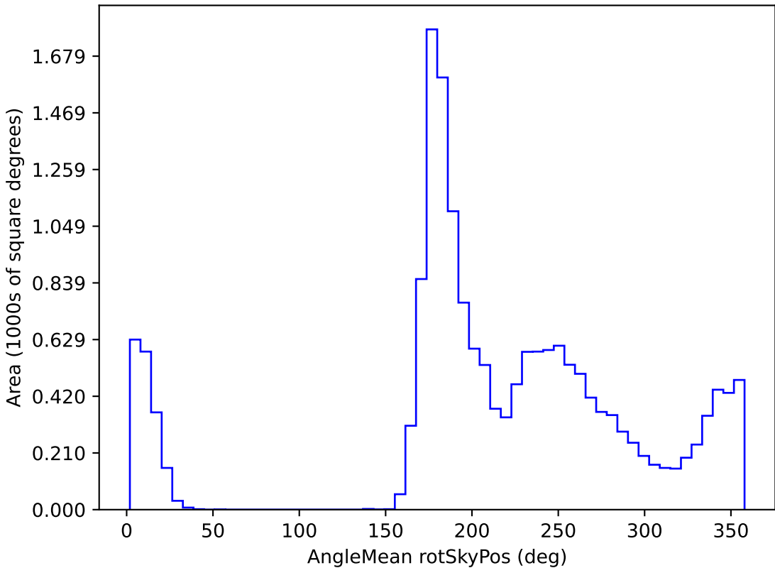
too_elab_r8_d2_griz_v3.4_10yrs WFD z band: AngleMean rotSkyPos
