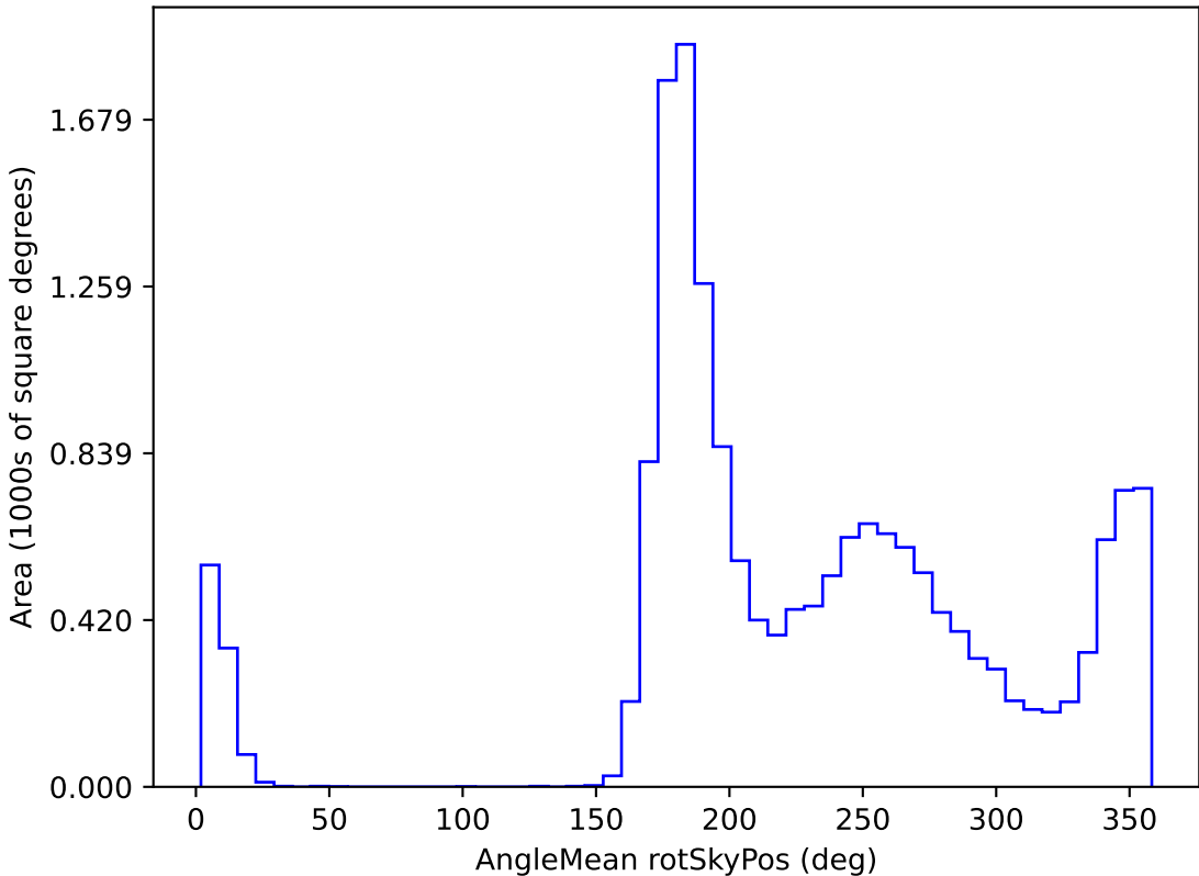
too_elab_r8_d2_griz_v3.4_10yrs WFD y band: AngleMean rotSkyPos
