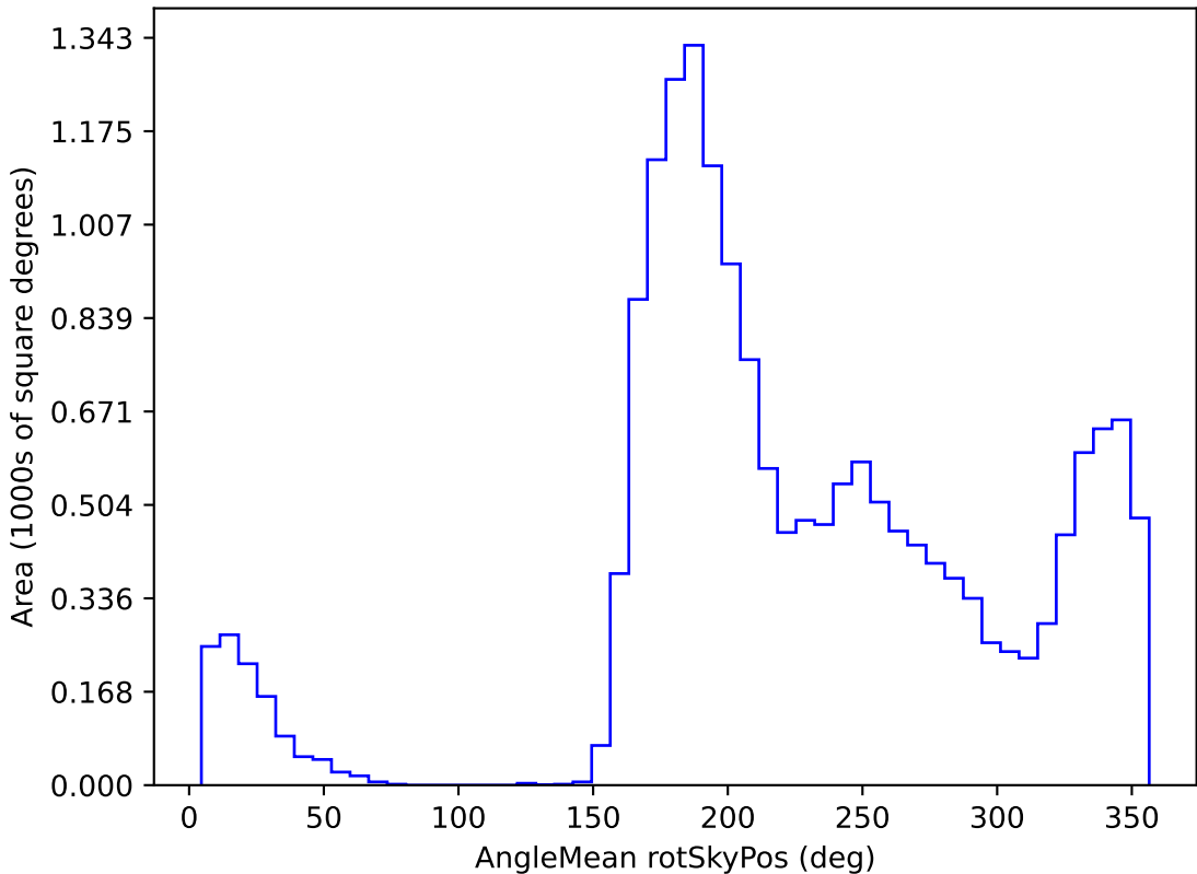
too_elab_r8_d2_griz_v3.4_10yrs WFD u band: AngleMean rotSkyPos
